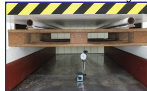
Bending Test
